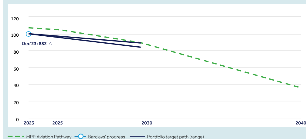
Financed emissions - Aviation (Passenger and Cargo) Physical Intensity (gCO 2 e/RTK) (Indexed December 2023 = 100)
