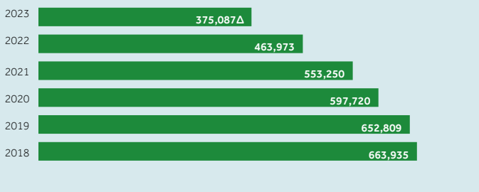
Total energy use (MWh)
