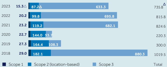
Total GHG emissions by Scope (location-based) '000 tonnes CO 2 e
