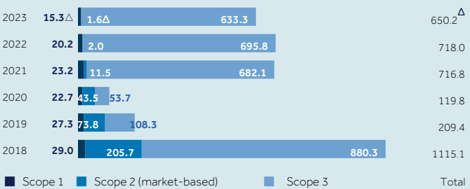
Total GHG emissions by Scope (market-based) '000 tonnes CO 2 e
